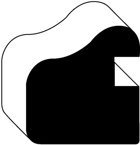
BAR RAIL STCH #3 • 3-3/8" x 3-1/2"
