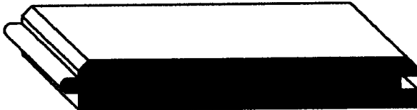
CLOSET LINER* STCH #130 • 5/16" x 3-3/8"
